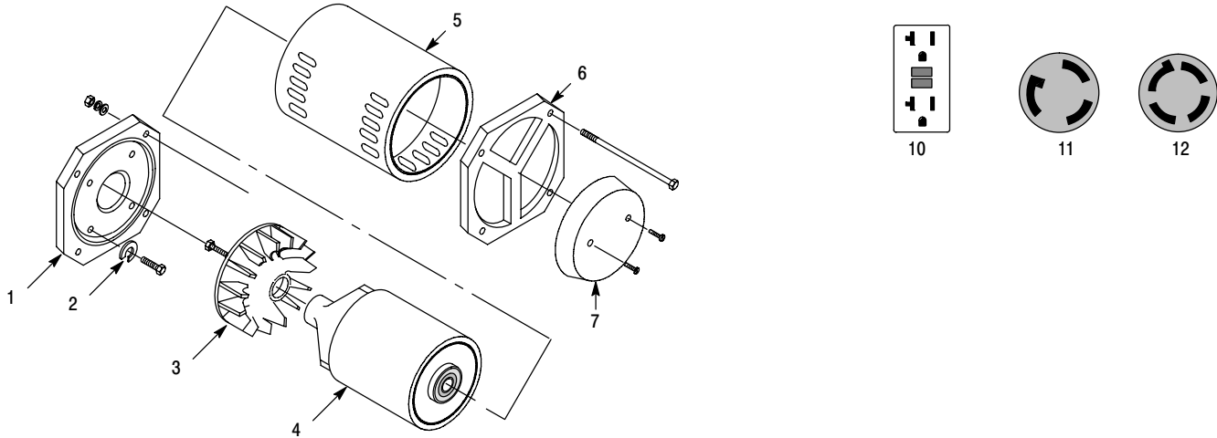
Figure A-3 Alternator Assembly
