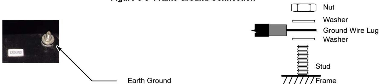
Figure 3-3 Frame Ground Connection
