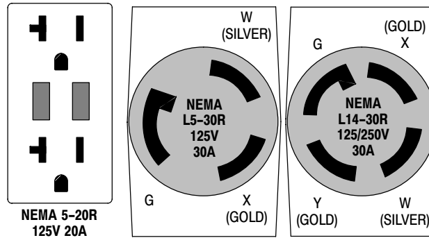
Figure 3-2 Receptacle Connections
