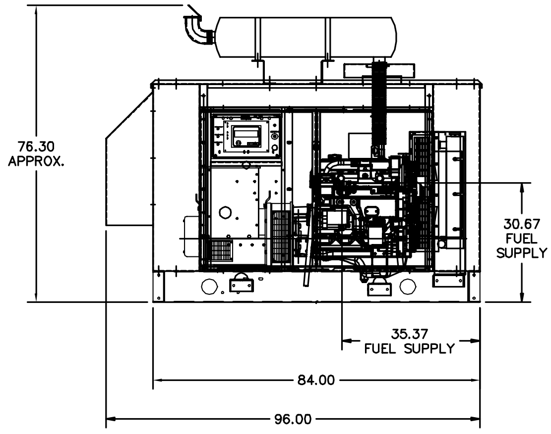
RIGHT VIEW
