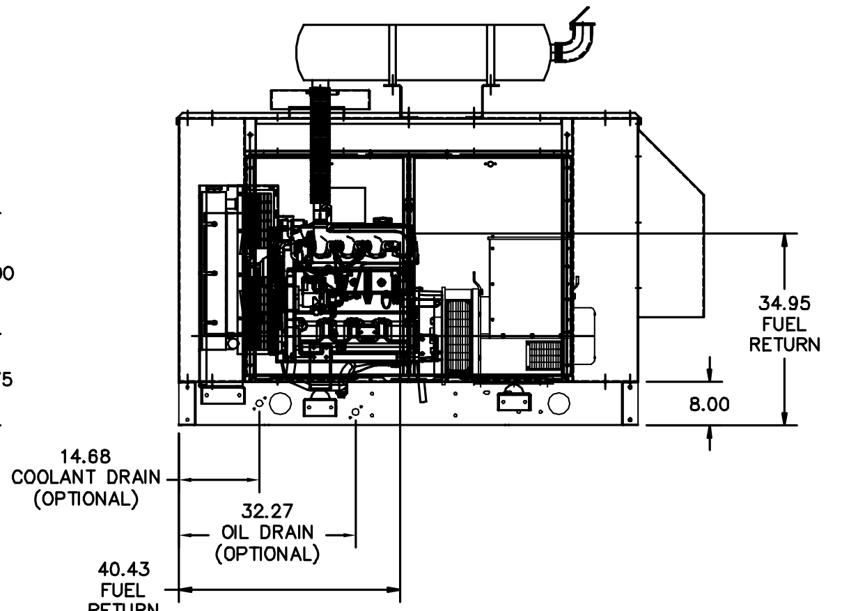
LEFT VIEW
