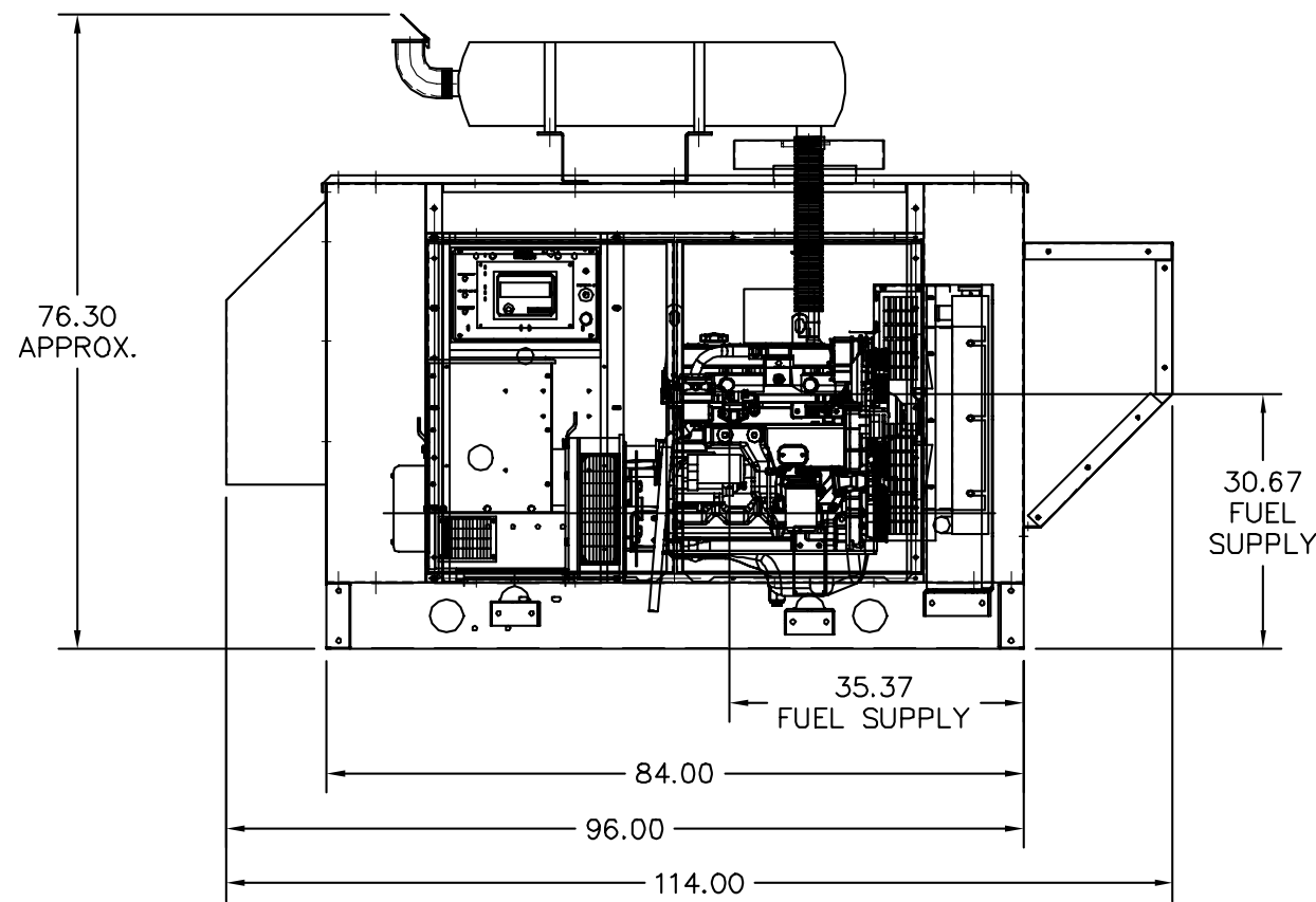
RIGHT VIEW
