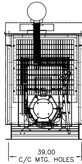
REAR VIEW
