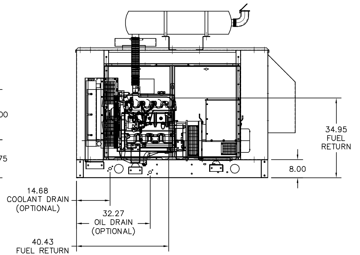
LEFT VIEW
