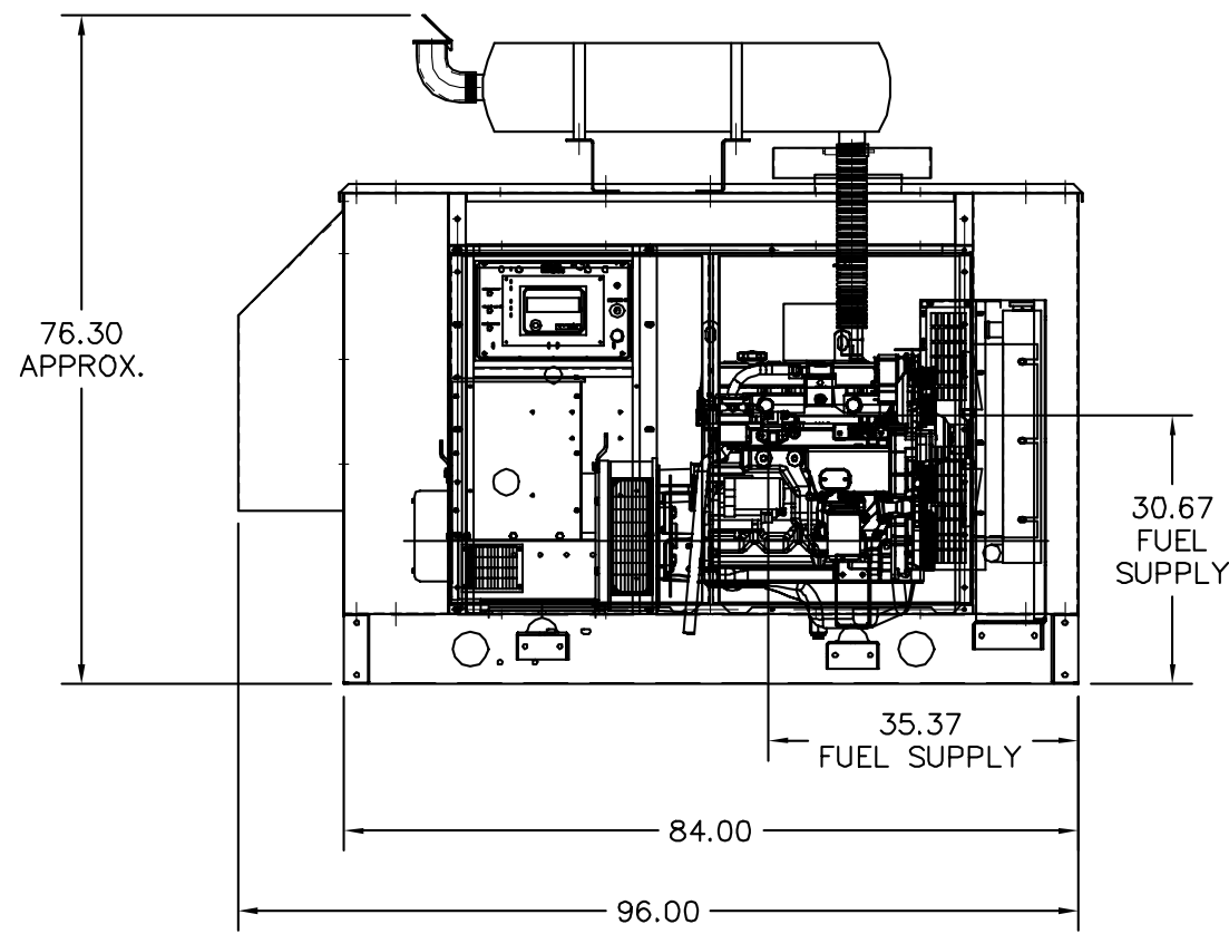
RIGHT VIEW
