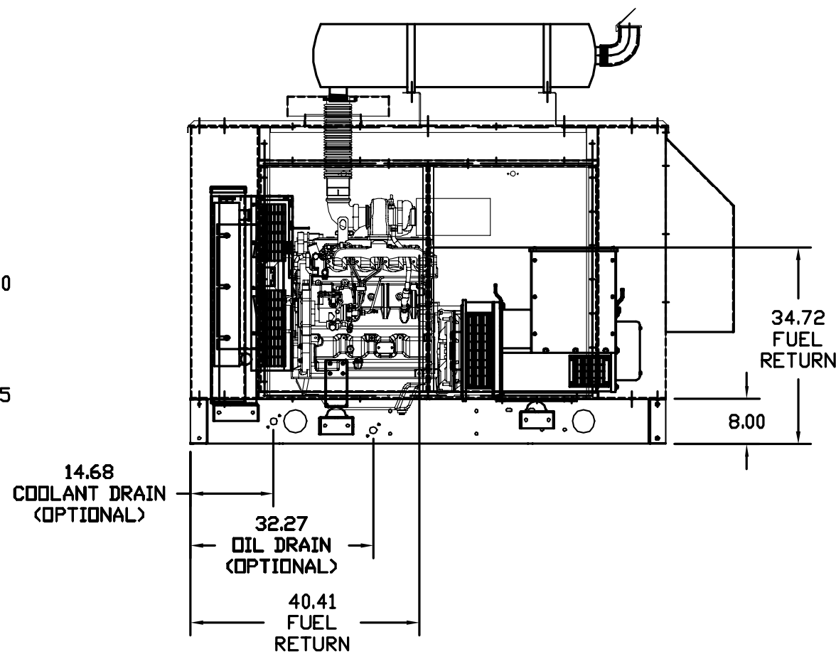
LEFT VIEW
