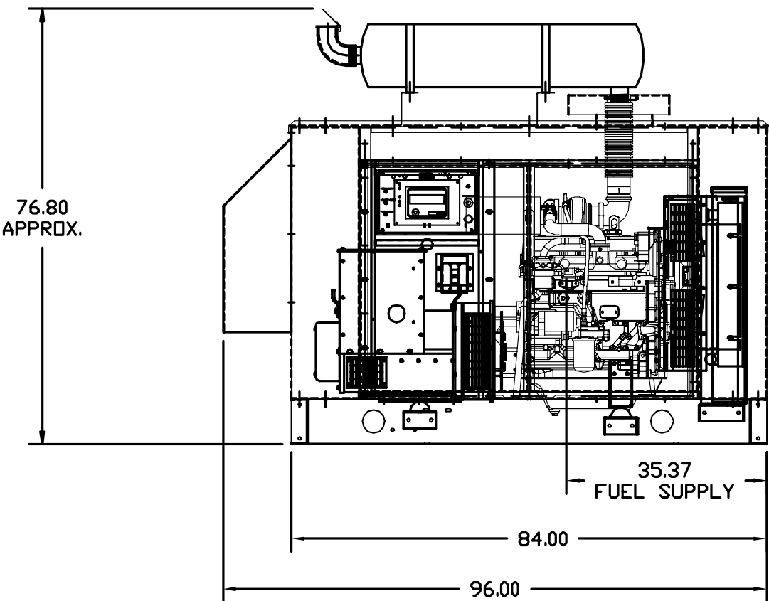
RIGHT VIEW
